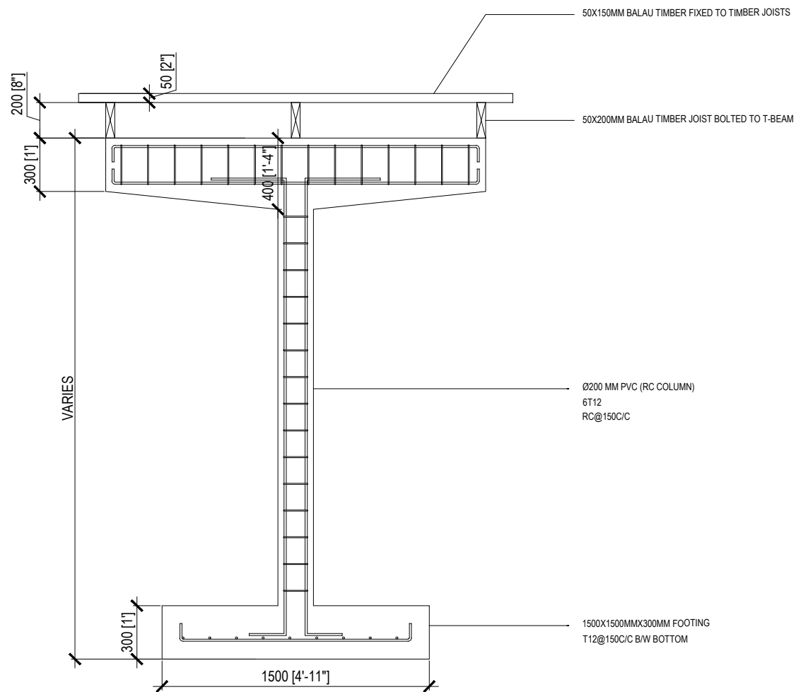
FOUNDATION/COLUMN/BEAM SECTION
