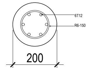
COLUMN C1 DETAIL
